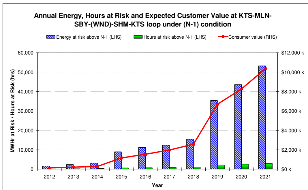
Figure 5: Energy at risk at KTS-MLN-SBY(WND)-SHM-KTS 66kV sub-transmission loop under N-1 condition (assuming a 50 th percentile demand)
