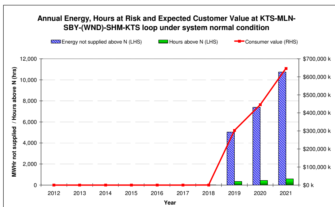
Figure 4: Energy not supplied at KTS-MLN-SBY(WND)-SHM-KTS 66kV sub-transmission loop under N condition (assuming a 50 th percentile demand)
